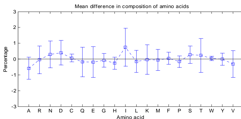
Fig. 2. Average amino acid difference in compositions of individual genes from the mesophilic to the psychrophilic temperature domain of 25 cytoplasmic proteins from the bacteria Vibrio . Bars are the empirical standard deviations.
