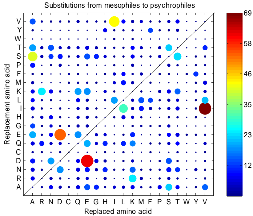
Fig. 3. Visualisation of all the pairwise substitutions between 25 sequences from the mesophilic (bottom) to the psychrophilic (left) group. The size and colour of the markers indicate the magnitude of the substitutions. Two clear trends can be seen: Val (V) is replaced by Ile (I), two sided mid-P-value=0.40; and Glu (E) is replaced by Asp (D), P-value=0.95. Many of the other minor changes are found to be statistically significant ( P < 0.05 ).
