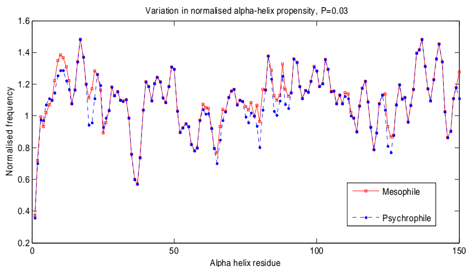
Fig. 5. Comparison of the mean helix formation parameter in the cytoplasmic protein Isocitrate lyase of 5 Vibrio gamma protobacteria (3 mesophilic and 2 psychrophilic). We used a box-filter of size m \times 3 as smoothing technique to recover the underlying structure in the data, where m is the number of sequences in the population. For this particular scale (Chou-Fasman, 1978) the helix-favourable values are at the positive y-axis. In average the mesophilic sequences appear to have more favourable values than the psychrophile counterparts.
